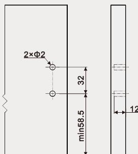
前面板钻孔尺寸 Front panel drilling dimension
