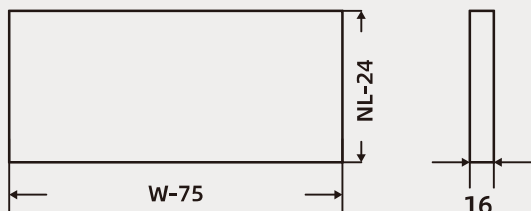
滑轨安装尺寸 Slide installation dimension
