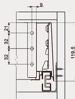
后背板开板尺寸 Rear panel cutting dimension
