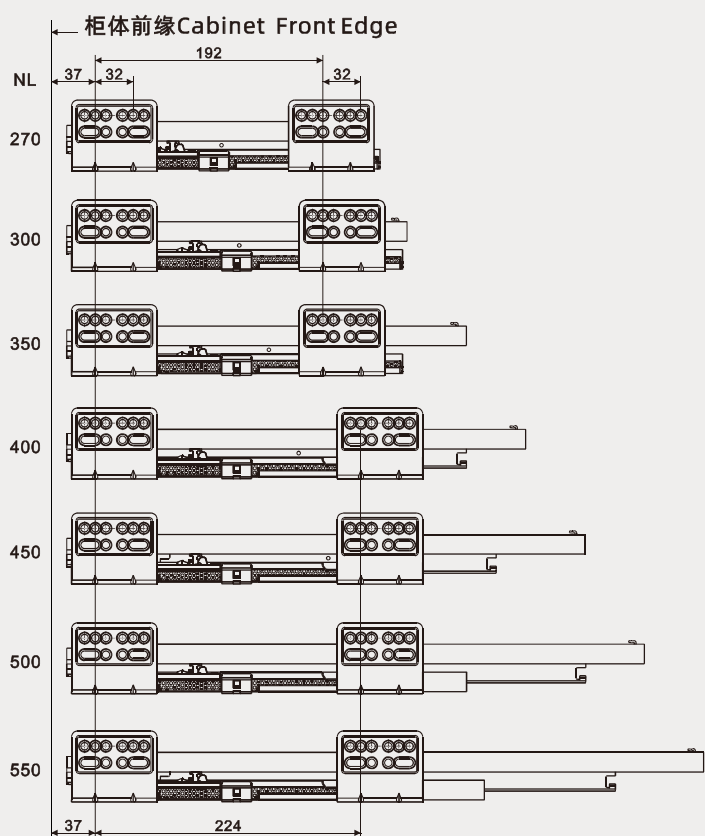
滑轨安装尺寸 Slide installation dimension
