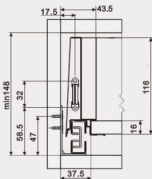
底板开板尺寸 Bottom panel cutting dimension
