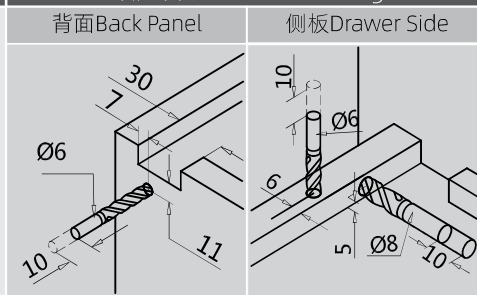
抽屉底部Drawer Bottom
